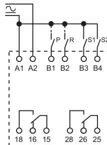
Wiring diagram
